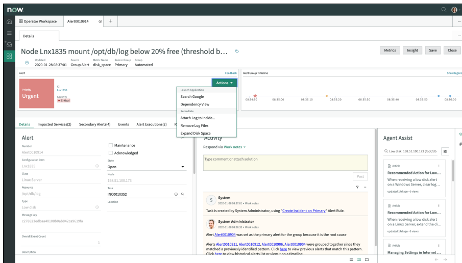
View business services impacted by a single alert
